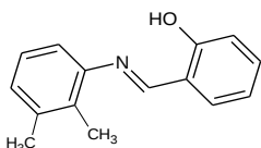
Fig. 1 Primary ligand 2-[(E)-[(2,3-dimethylphenyl)imino]methyl]phenol
