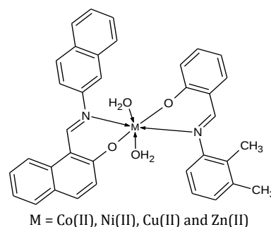
Fig. 4 The metal-ligand ternary binding proposed structure
