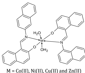
Fig. 3 The metal-ligand binary binding proposed structure
