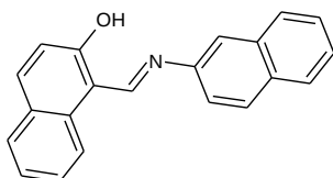
Fig. 2 Secondary ligand 1-[(E)-(naphthalen-1-ylimino)methyl]naphthalen-2-ol
